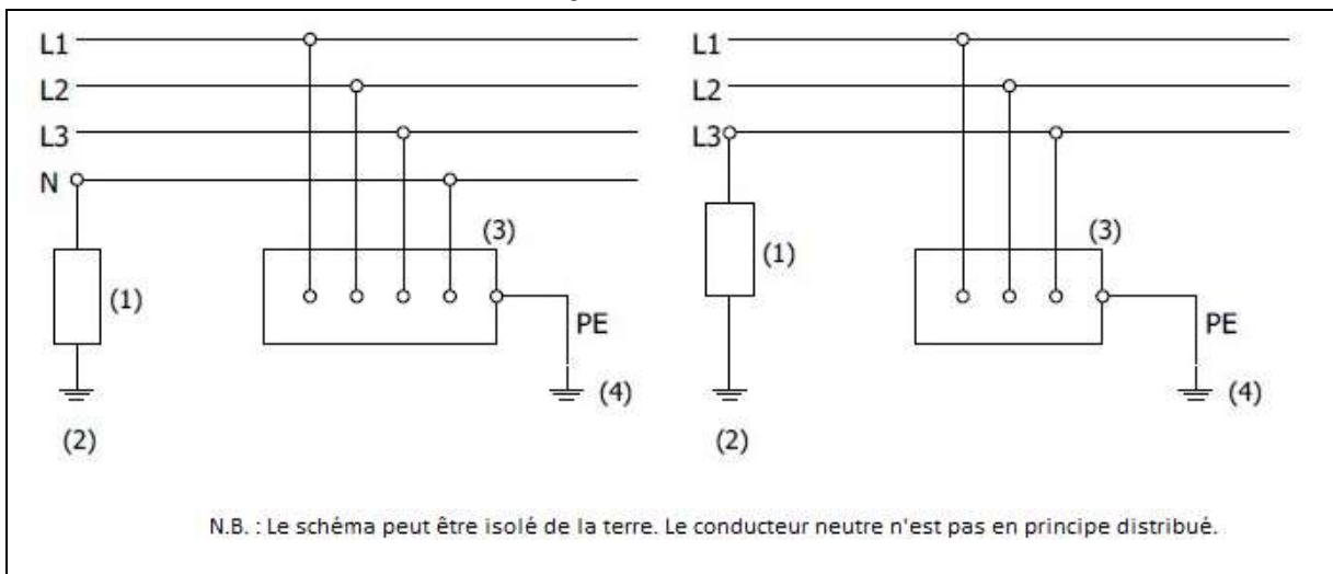
Figure 3.5. Schéma IT
