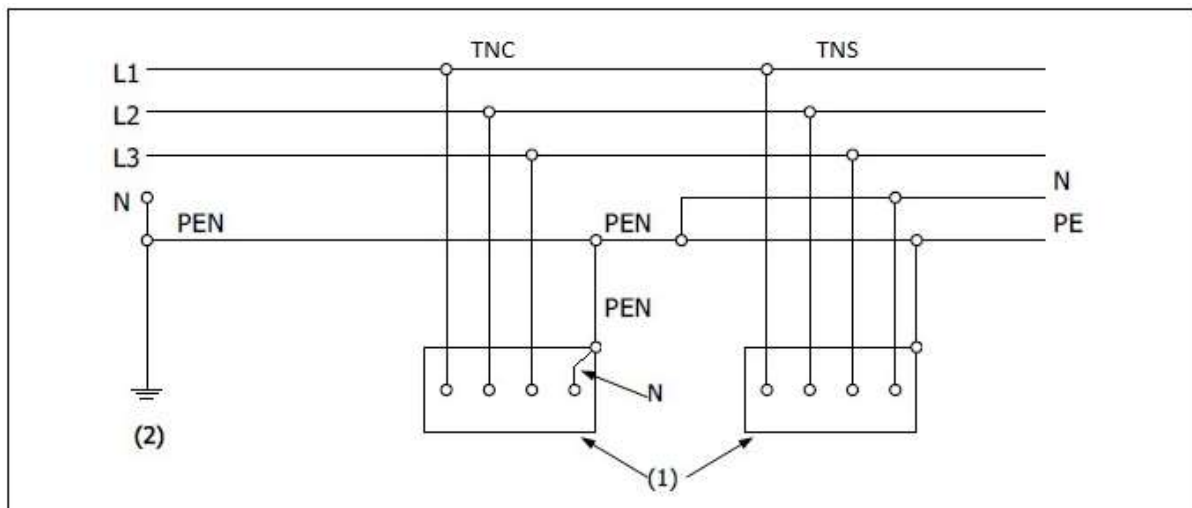
Figure 3.3. Schéma TN-C-S
