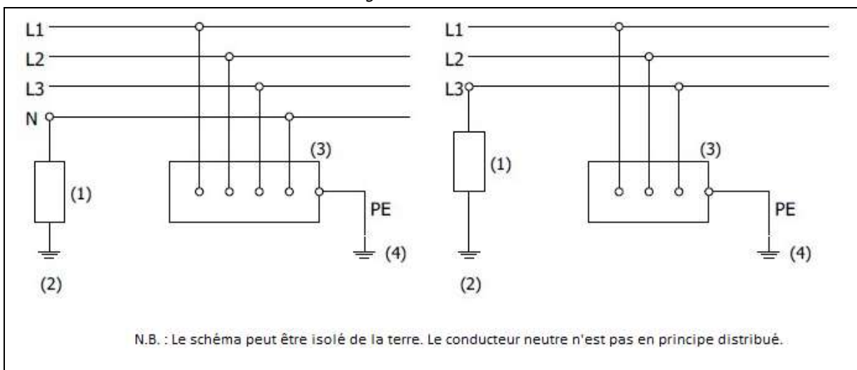
Figure 3.5. Schéma IT
