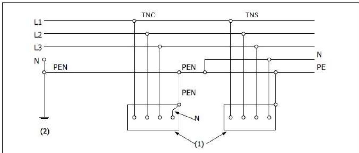
Figure 3.3. Schéma TN-C-S
